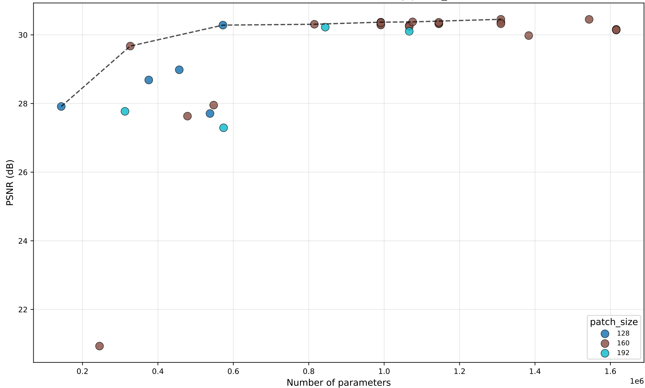
PSNR vs #Params — SRFormer — by patch_size
